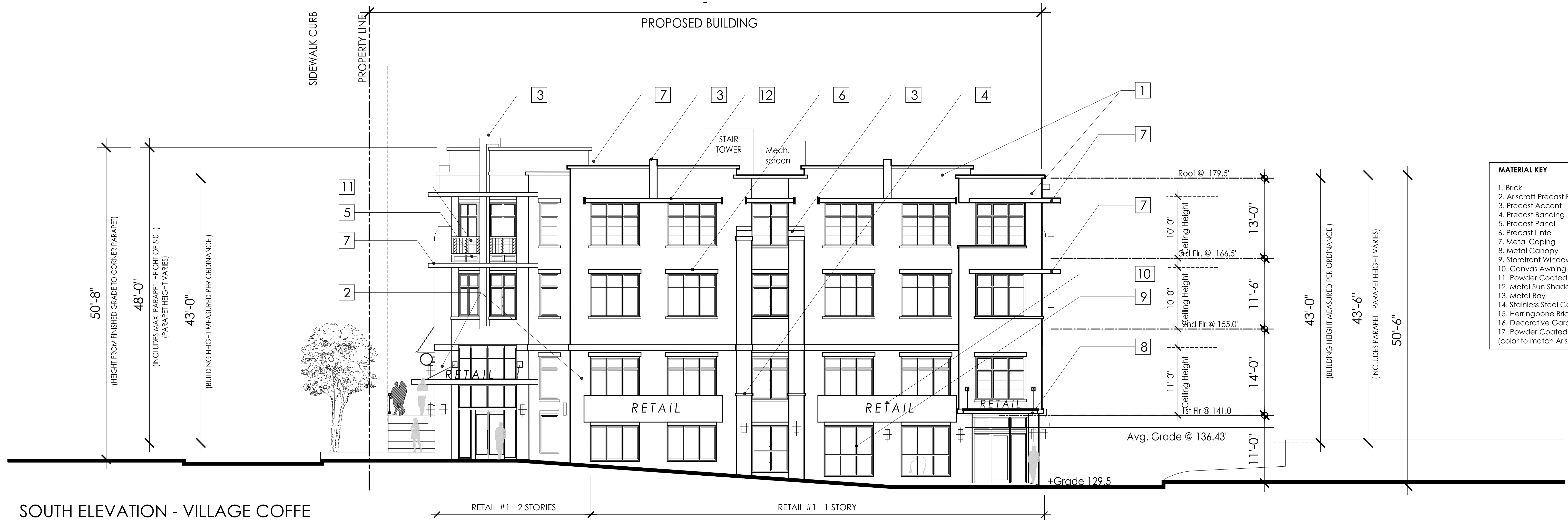
SOUTH ELEVATION - VILLAGE COFFE SCALE: 1/8" = 1'-0"
